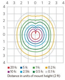
FG 6LED ISOFOOTCANDLE PLOT
